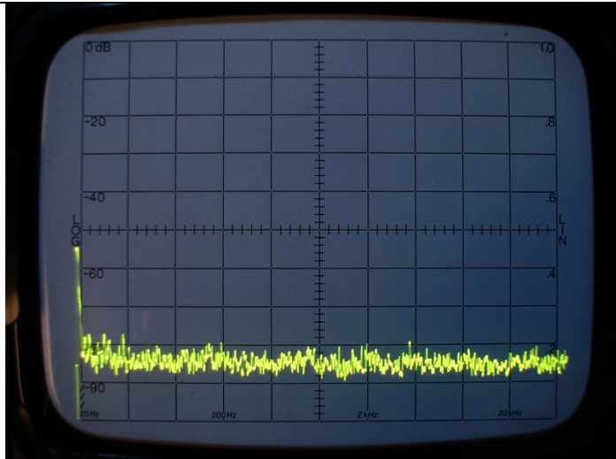
Noise 0 → 10kHz – Ref : - 40 dBV
